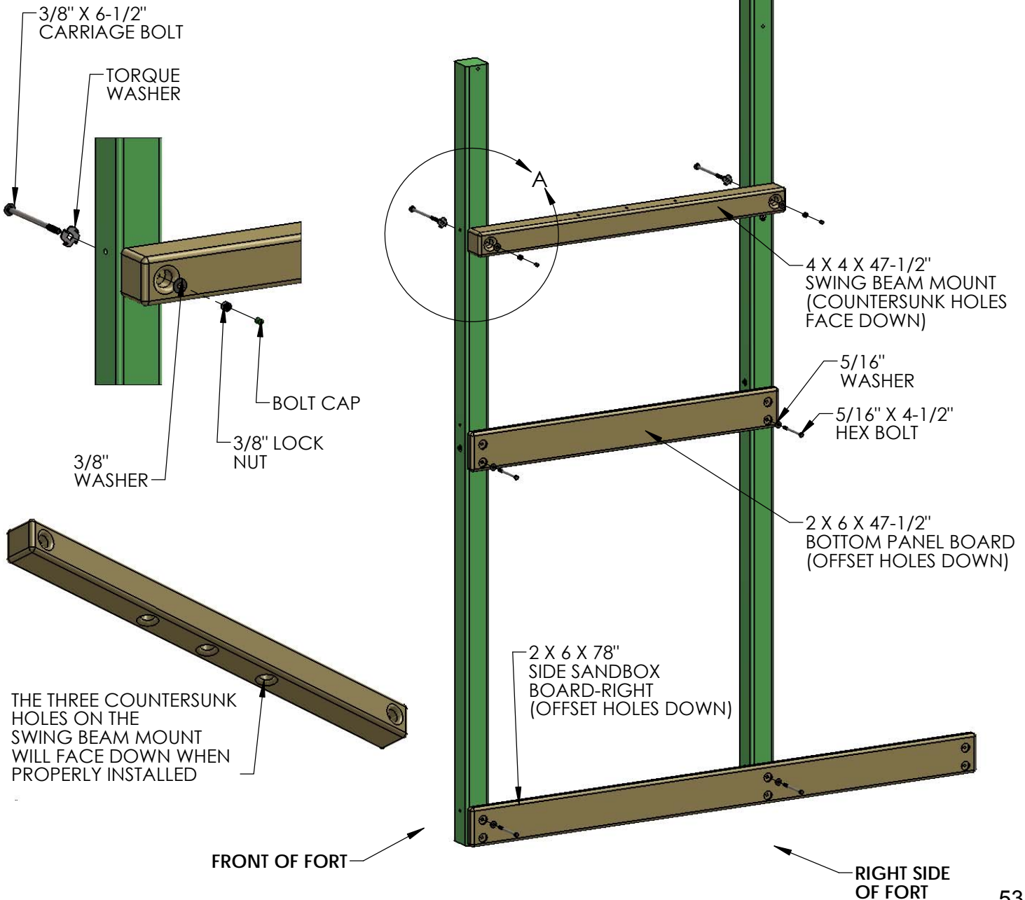
DETAIL A
